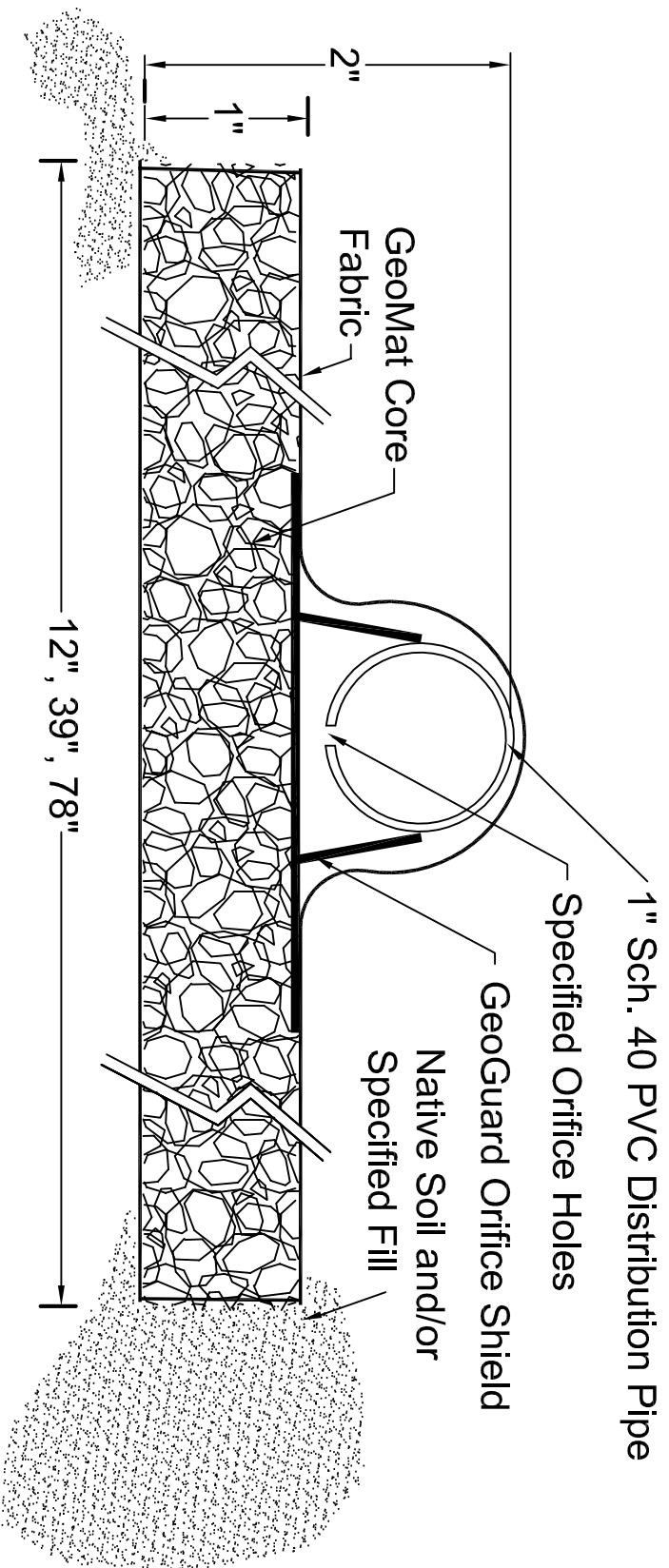
GEOMAT LEACHING SYSTEM Cross Section - Not to Scale -
